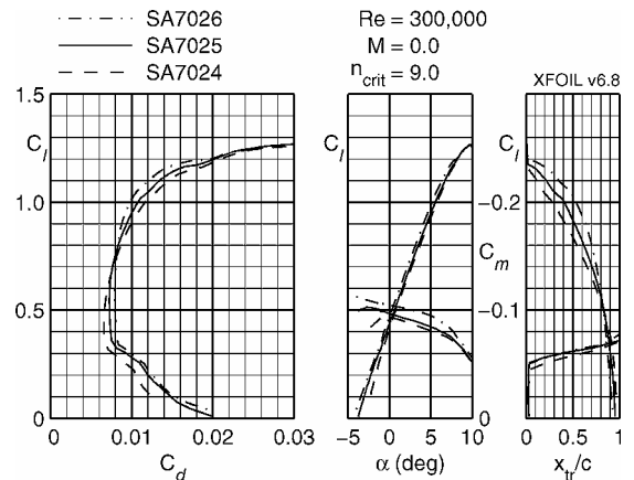
Fig. 10 XFOIL predictions for the SA702x airfoil series at Re of 300,000.
